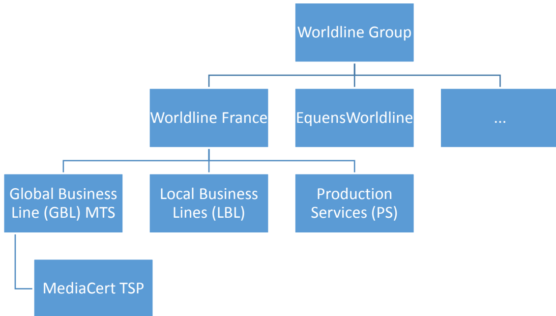
Figure 2 - Organizational diagram
